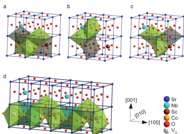
Figure 4. Transport paths for different oxygen vacancy defects in a SrSc 0.125 Nb 0.125 Co 0.75 O 3-δ model. a) V O [Sr 4 Co 2 ], b) V O [Sr 4 CoNb], c) V O [Sr 4 CoSc]. The path of V O [Sr 4 Co 2 ] with the lowest migration barrier is depicted in (d).
